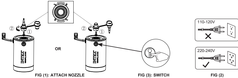
FIG (1): ATTACH NOZZLE
